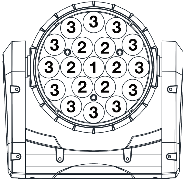
Pixel Zone Layout 28 Ch. Mode (29 Ch. Mode w/ Software Version \geq 1.6 )
