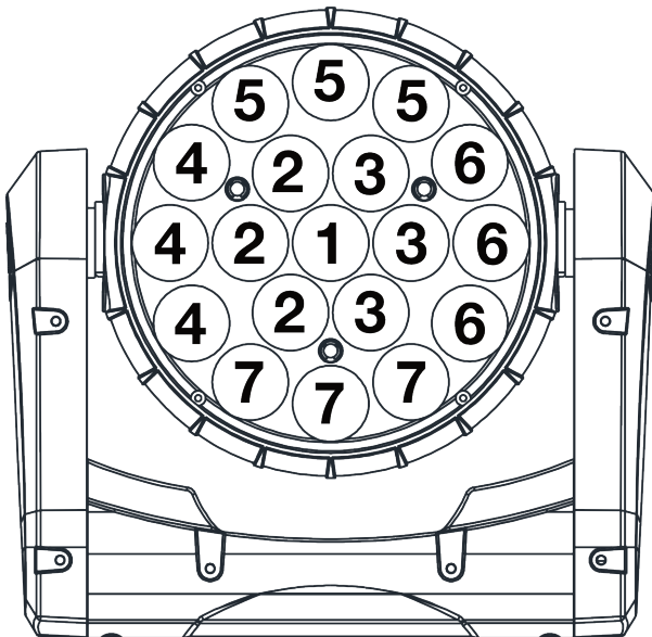
Pixel Zone Layout 44 Ch. Mode (45 Ch. Mode w/ Software Version \geq 1.6 )
