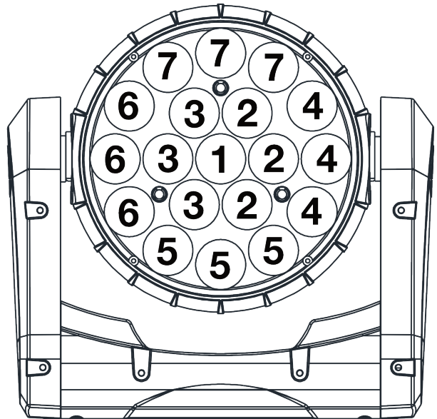
Pixel Zone Layout 44 Ch. Mode (45 Ch. Mode w/ Software Version \geq 1.6 )
